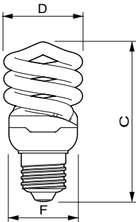
QSPIR-F T2 12W/827 E27 220-240V 50/60Hz
